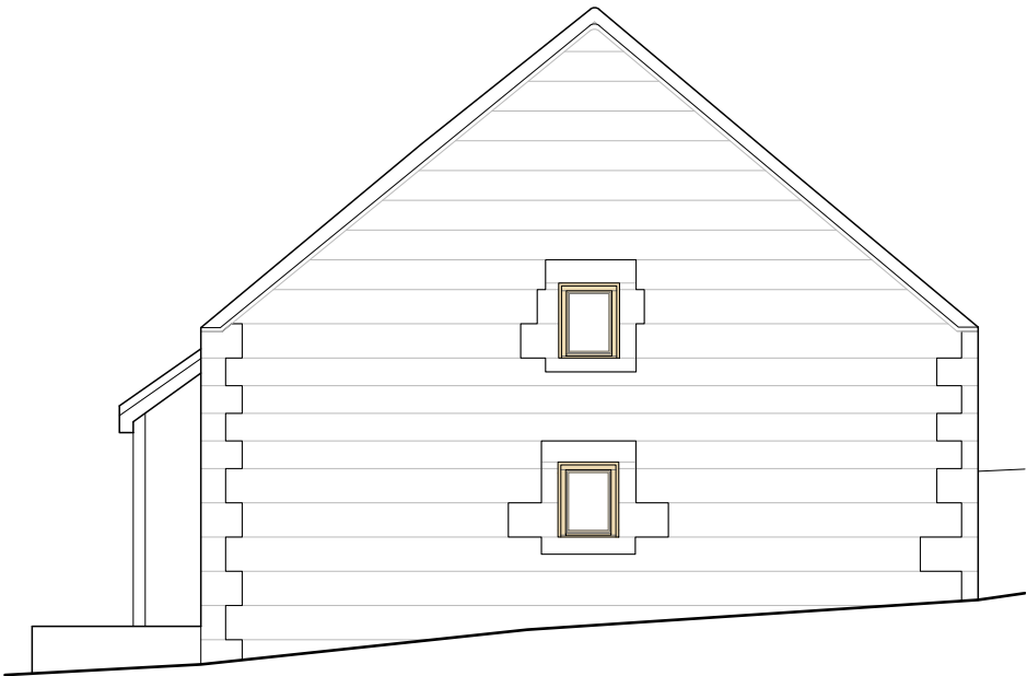
ALAN STEVENSON HOUSE NORTH WEST ELEVATION
